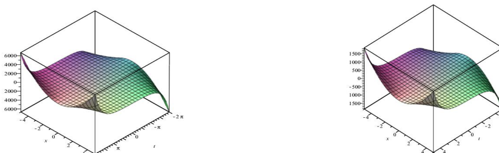
Figure 5: Surface plot for approximate solution for Example 2
