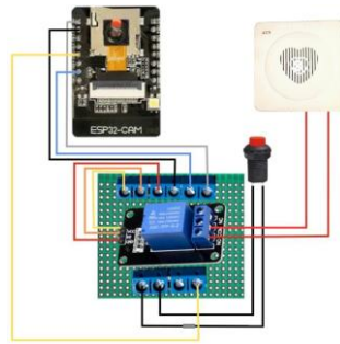
Gambar 3 Wiring Diagram Sistem
