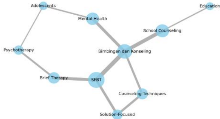
Gambar 1. Jaringan VOSviewer
