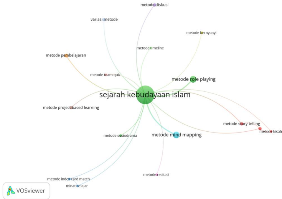
Gambar 4 Network Visualization
