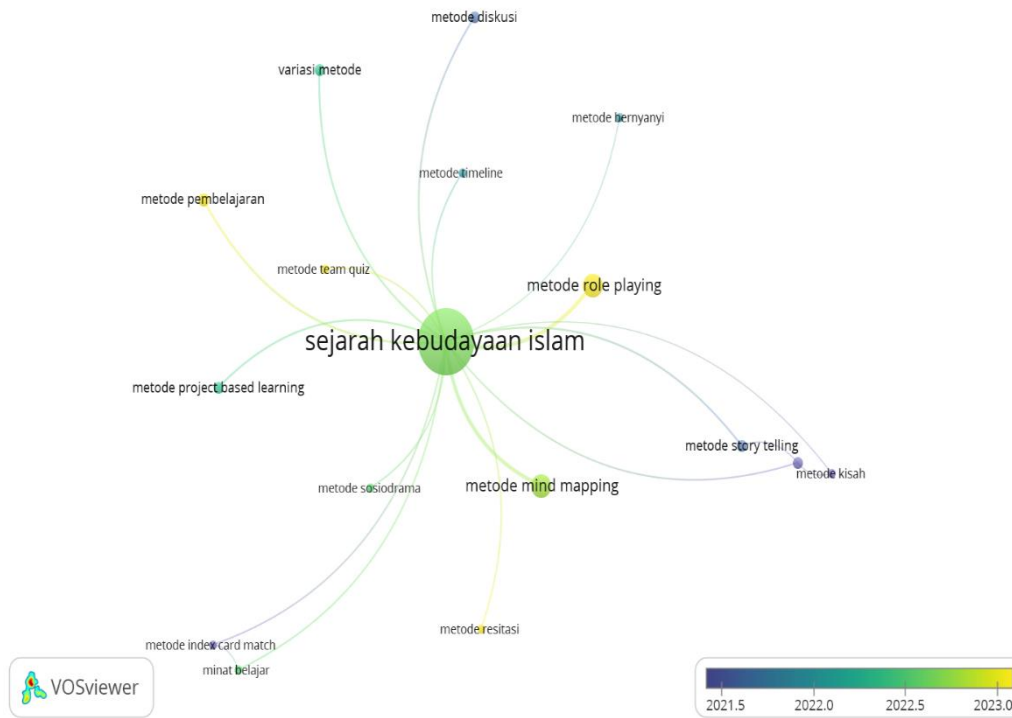
Gambar 1 Overlay Visualization
