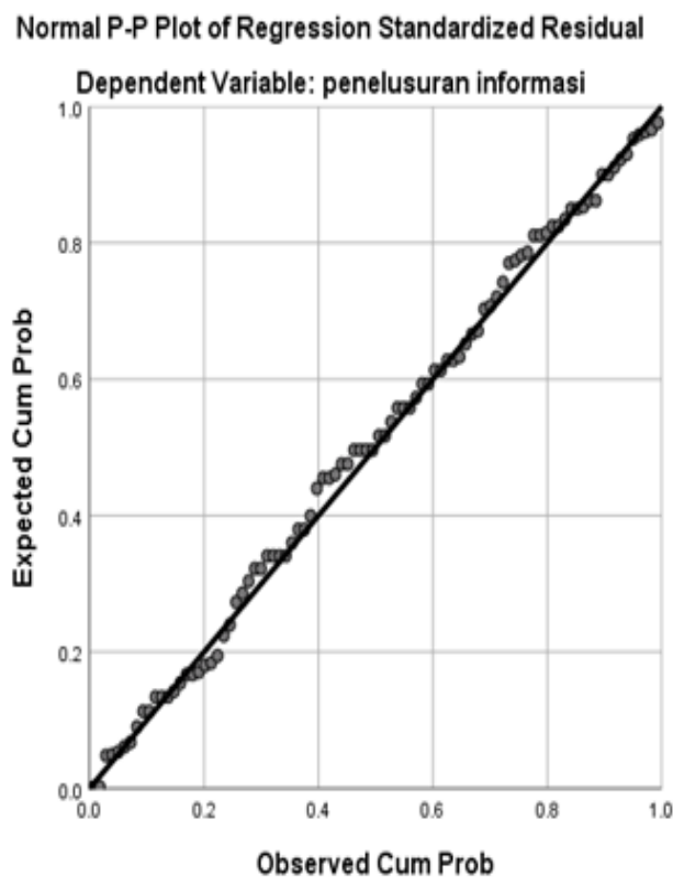
Gambar 1. Normal Probability Plot
