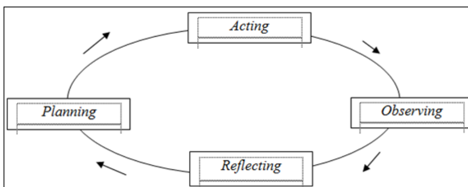
Gambar 2. Model Kurt Lewin (Sumber Educate by Rima, 2021)
