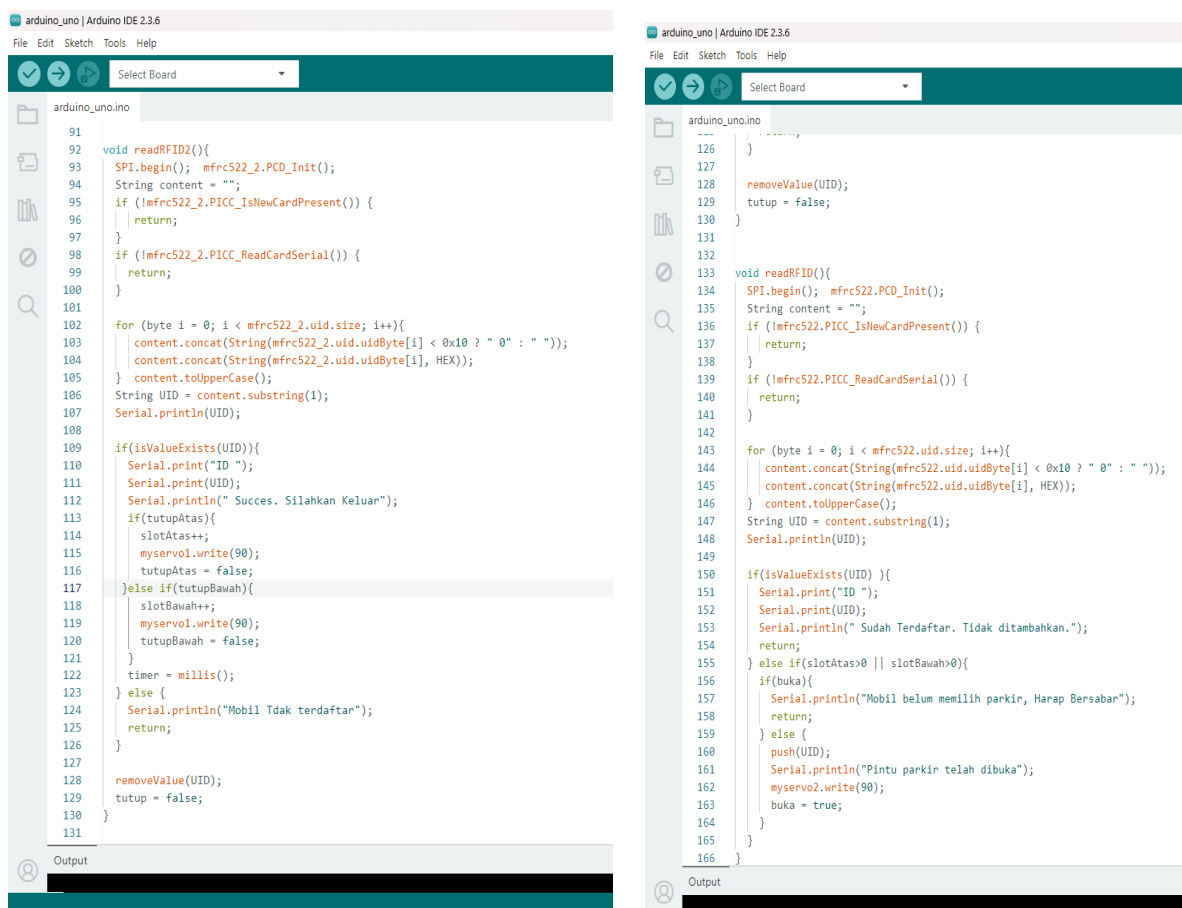
Gambar 1. Program RFID
