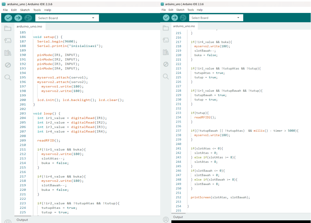
Gambar. 5 Listing Program Motor Servo
