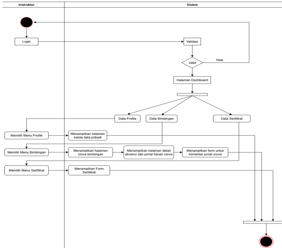
Gambar 5. Rancangan Diagram Activity Instruktor
