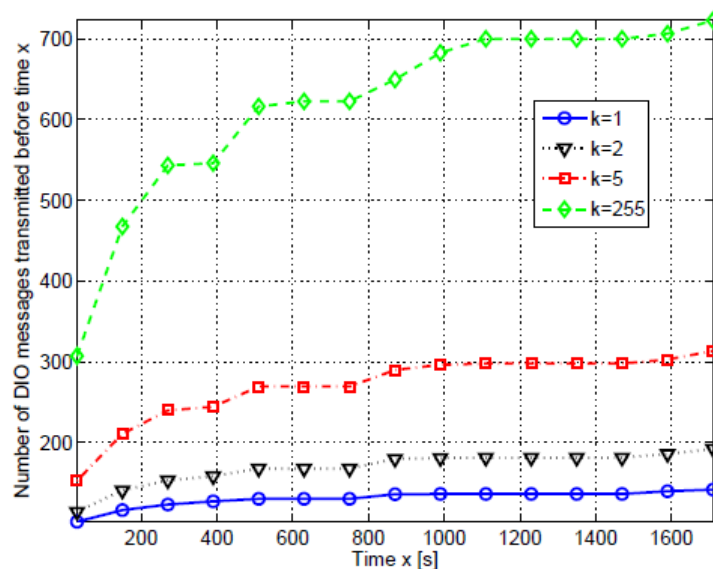
Figure 4. Number of DIO messages transmitted in the network over time.
