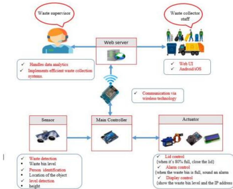
Figure 11: Architectural Design
