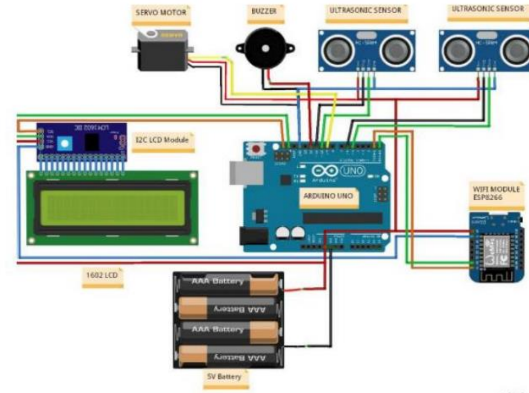
Figure 10: Schematic Diagram
