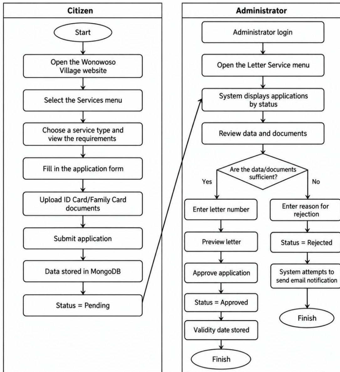
Figure 2. Flowchart of Wonowoso Village Mail Service System
