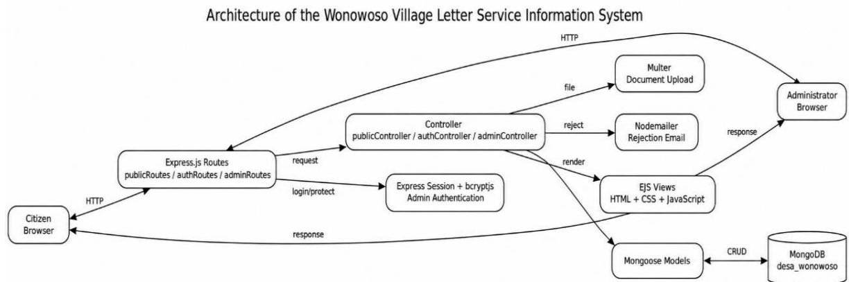
Figure 1. Letter Service Information System Architecture
