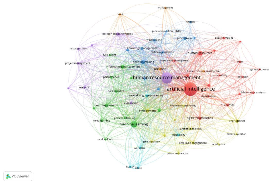
Figure 4. Network Visualization
