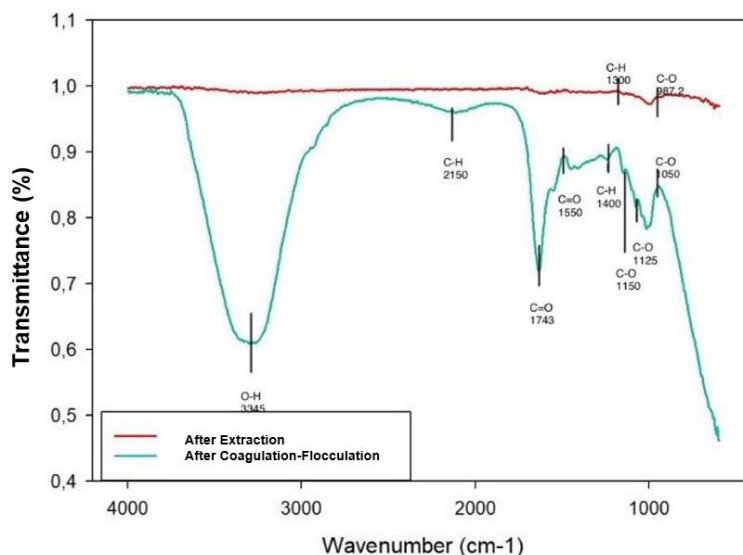
Figure 6. FTIR result
