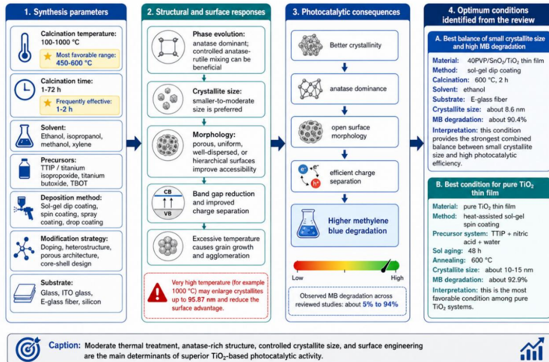
Figure 2. Schematic of the relationship between synthesis parameters, morphostructural characteristics, and photocatalytic activity of TiO 2 -based thin films
