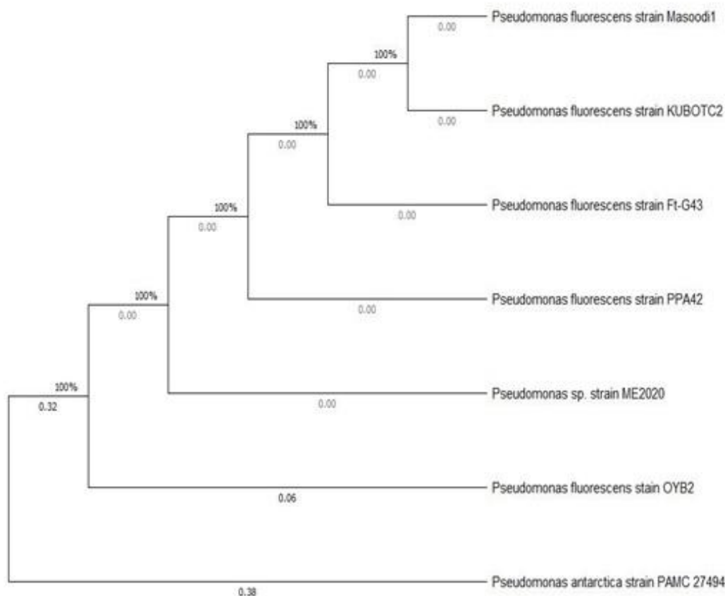
Figure 2: Phylogenetic tree of bacterial isolates constructed using Neighbor-Joining method (MEGA 11)
