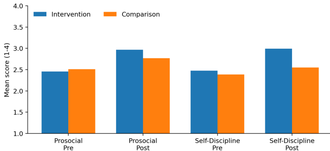
Figure 1. Mean Pretest and Posttest Scores by Group in the Simulated Dataset
