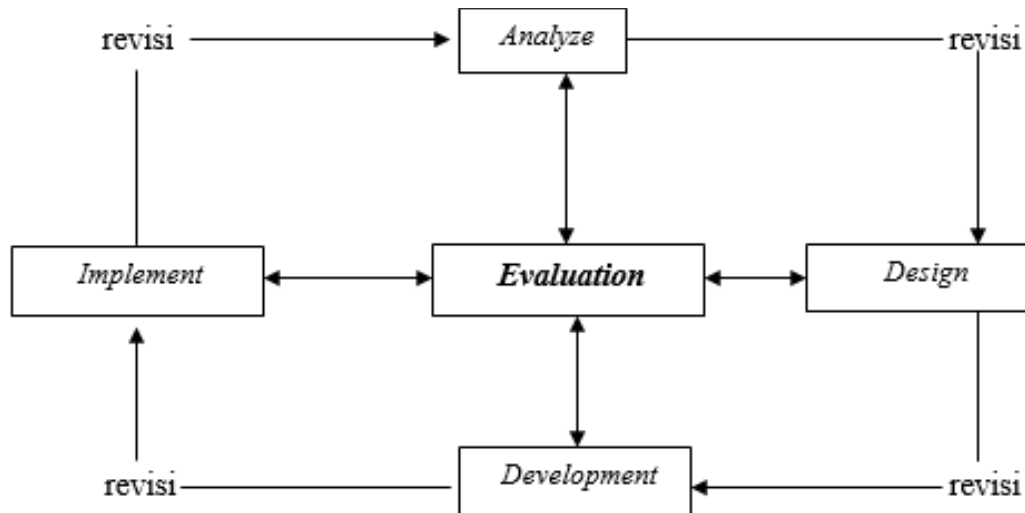
Gambar 1 model ADDIE
