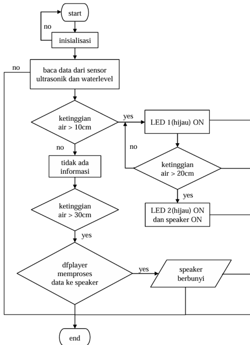
Gambar 2. Flowchart
