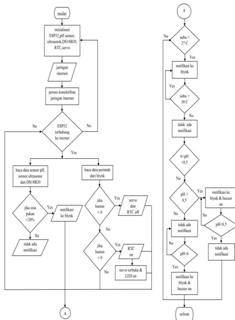
Gambar 2. Flowchart Alat
