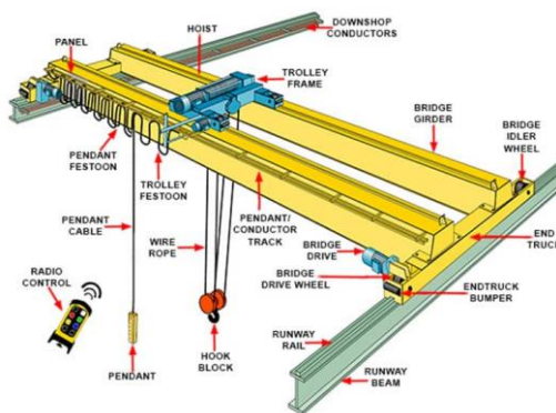
Gambar 1. Hoist crane
