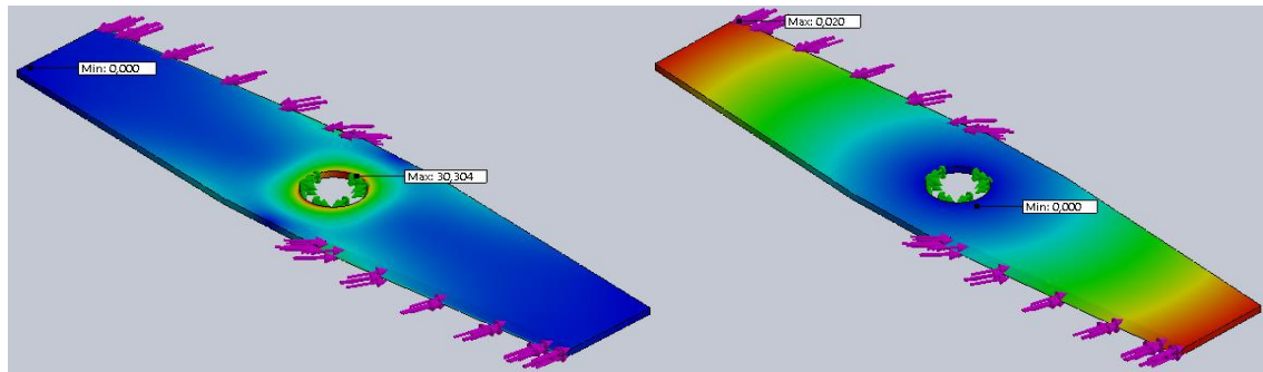
Gambar 9. Stress and displacement Result 33°
