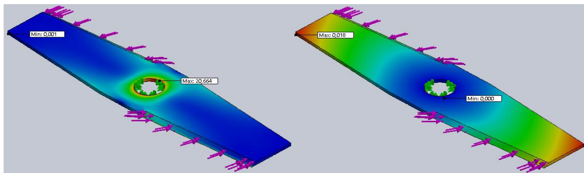
Gambar 9. Stress and displacement Result 31^{\circ}
