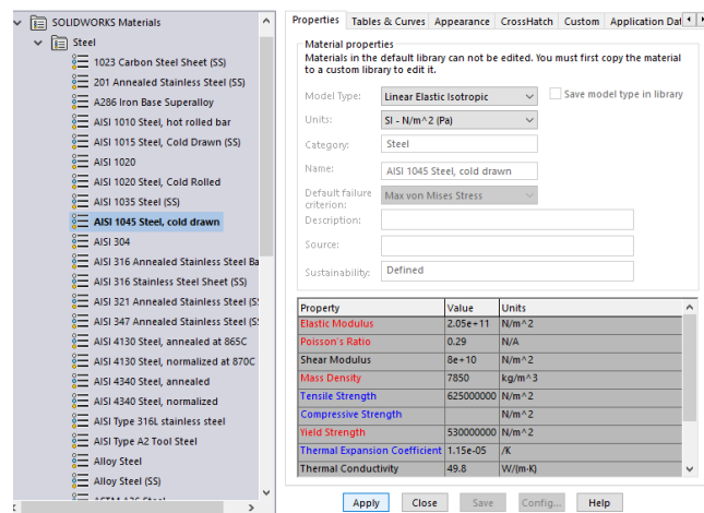
Gambar 3. Applay Material 1045 Steel Cold Drawn
