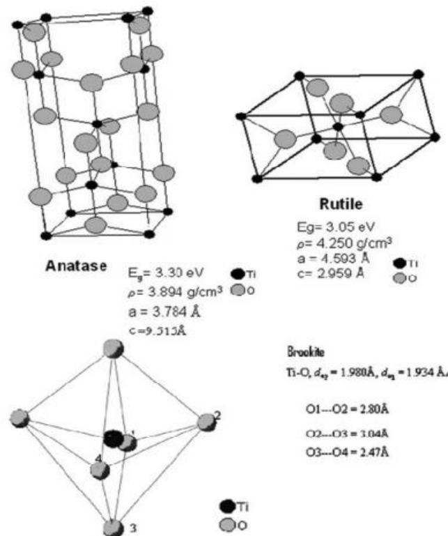
Gambar 1 Struktur Fasa Kristal \text{TiO}_2 (Macwan et al., 2011)
