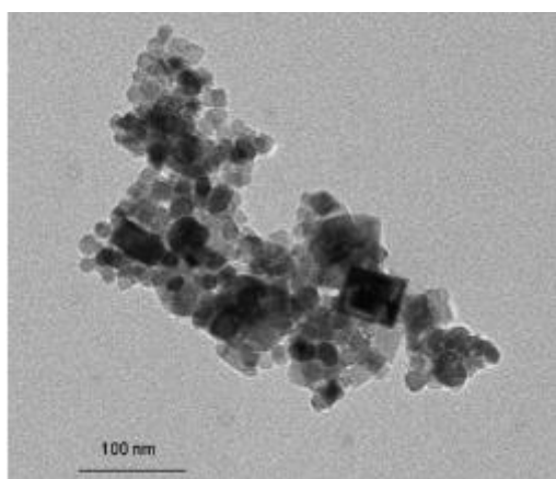
Gambar 4 Morfologi TEM partikel nano \text{TiO}_2 metode solvotermal (Wahi et al., 2006).
