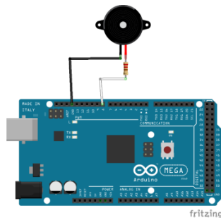
Gambar 13. Rangkaian Buzzer
