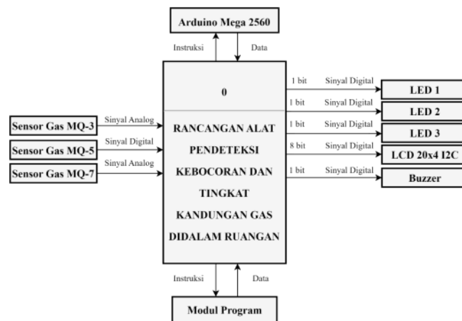
Gambar 2. Context Diagram
