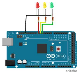
Gambar 12. Rangkaian LED
