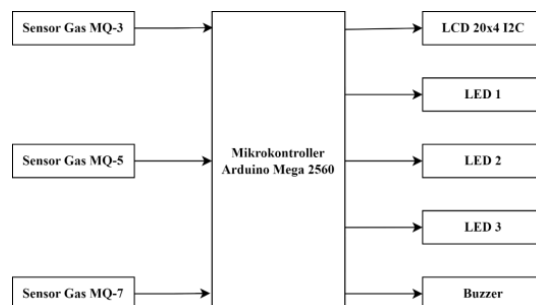
Gambar 4. Blok Diagram
