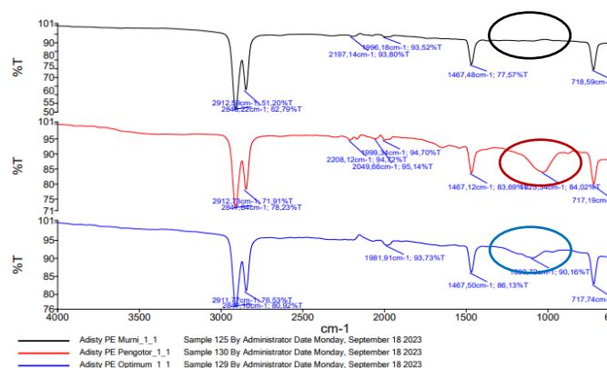
Gambar 2. Hasil Split Garis FTIR
