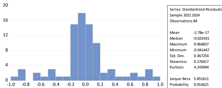
Gambar 1. Histogram
