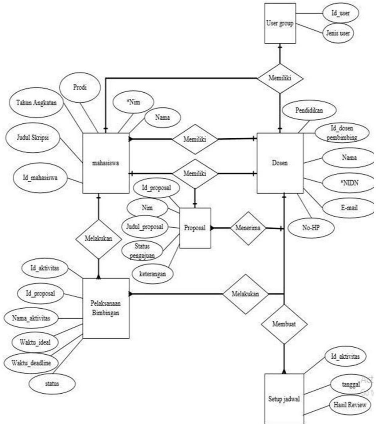
Gambar 3. Entity Relationship Diagram (ERD)
