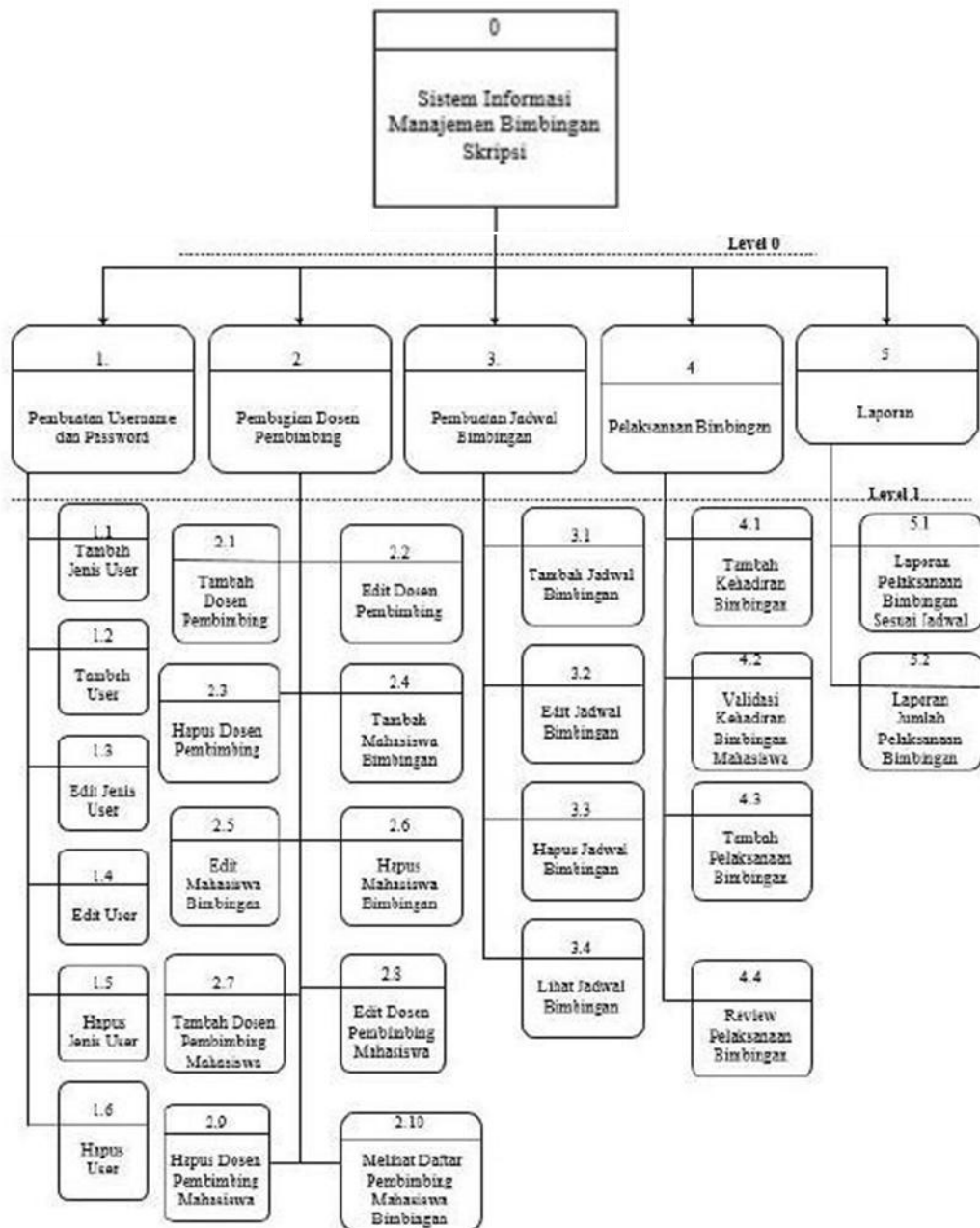
Gambar 2. Diagram Data Flow (DFD) Level
