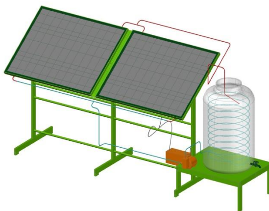
Gambar 2. Alat Collector Thermal Surya
