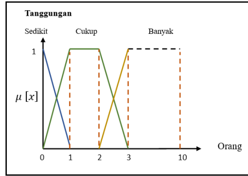
Figure 3. Fuzzy Set Curve for Dependents
