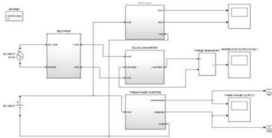
Figure 1: Block Diagram
