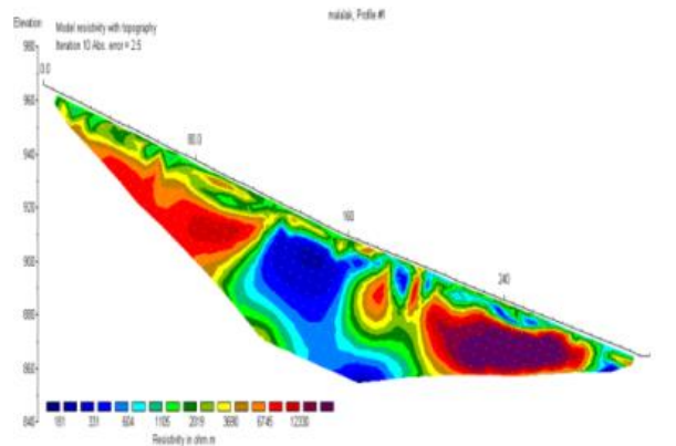
Fig 6. Distribution of resistivity and path depth 5
