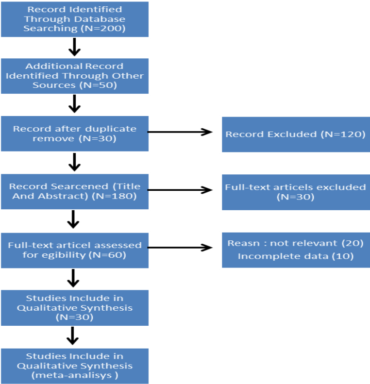
Figure 1. PRISMA Flowchart
