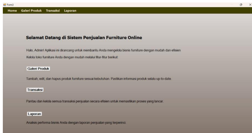
Gambar 3 Halaman Dashboard
