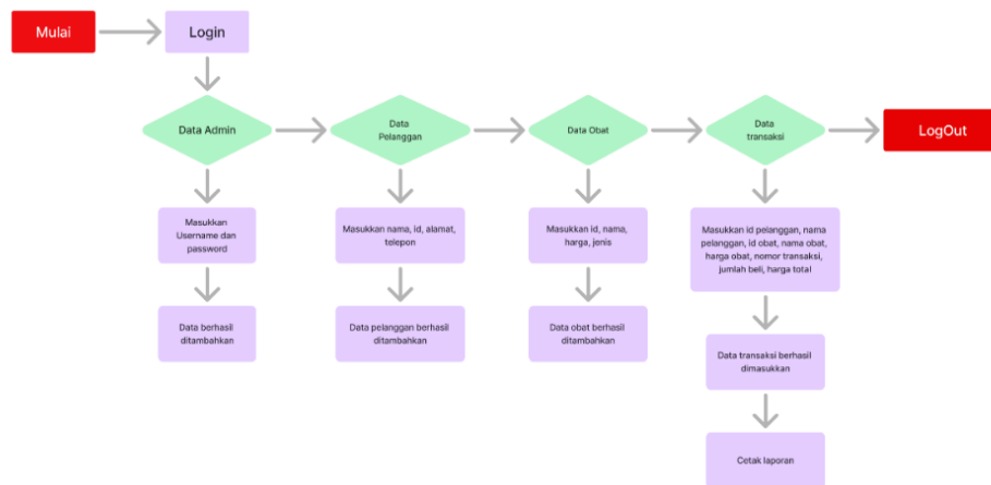
Gambar 1: flowchart
