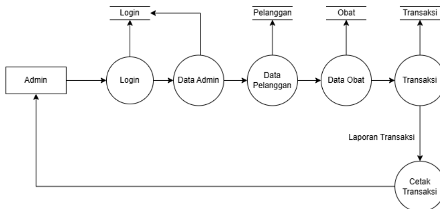
Gambar 2: diagram DFD
