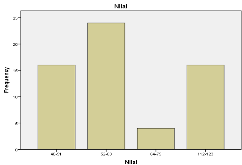
Gambar 1. Diagram distribusi frekuensi variabel X
