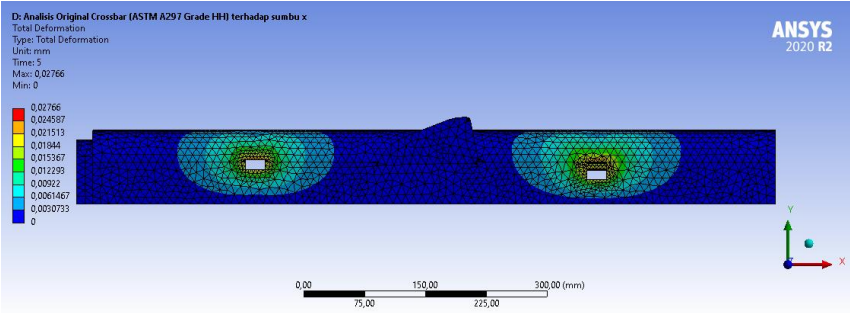
Gambar 8 Contoh hasil simulasi total deformation (displacement) mm.
