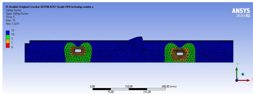
Gambar 9. Contoh hasil simulasi safety factor.
