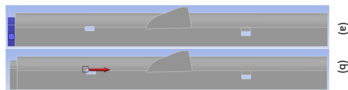
Gambar 5 (a) Lokasi Fixed support, (b) Arah gaya pembebanan
