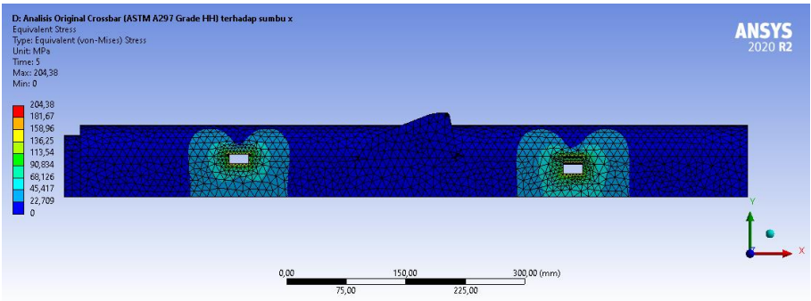
Gambar 7 Contoh hasil simulasi equivalent (Von Mises) stress (mpa).
