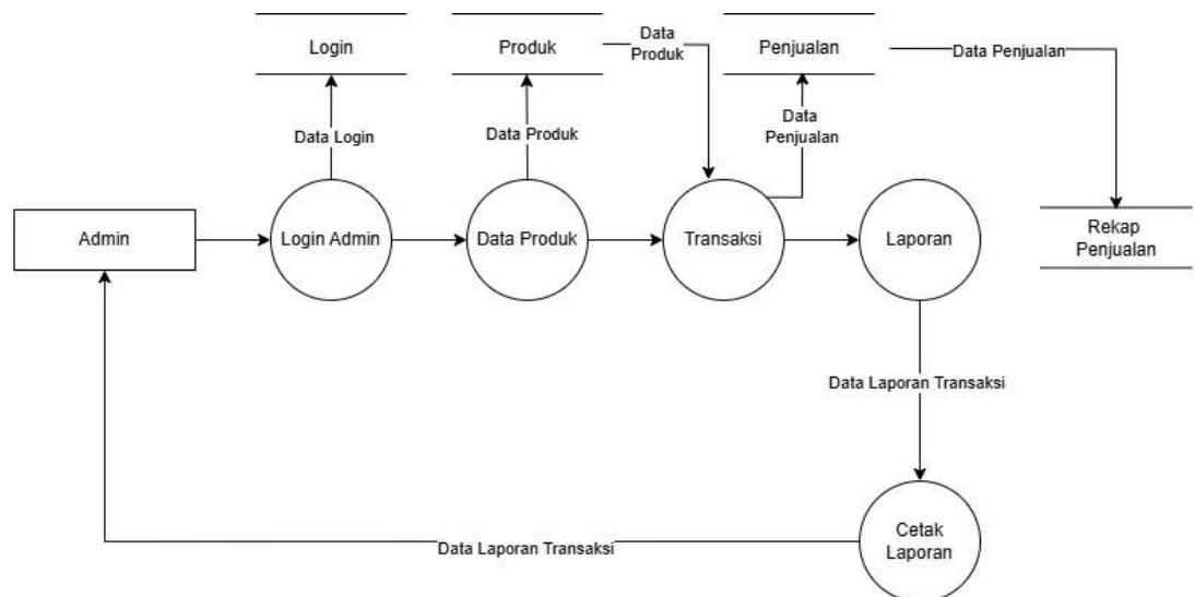
Gambar 1 Data Flow Diagram
