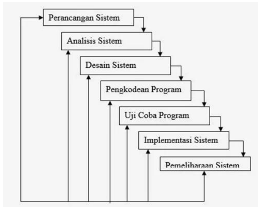
Gambar 1 . Metode Waterfall
