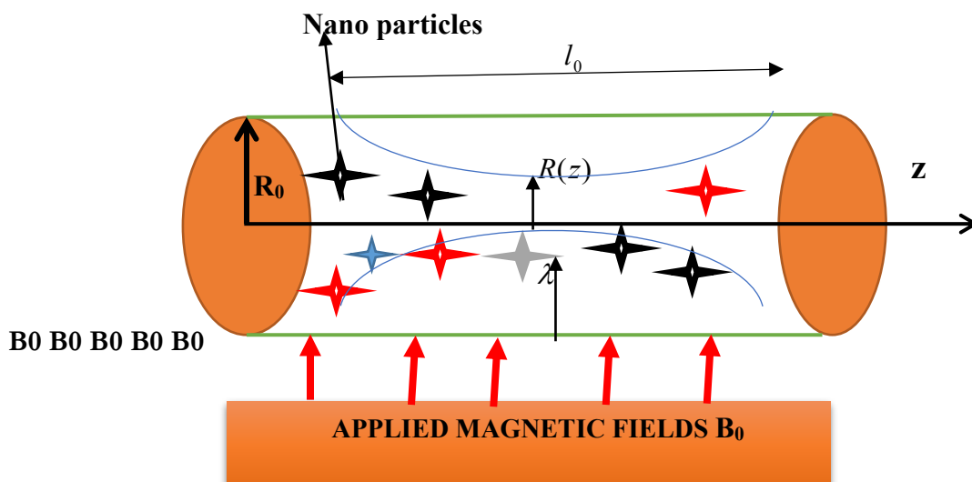
Figure 1: Flow Geometry of the Stenosed Artery
