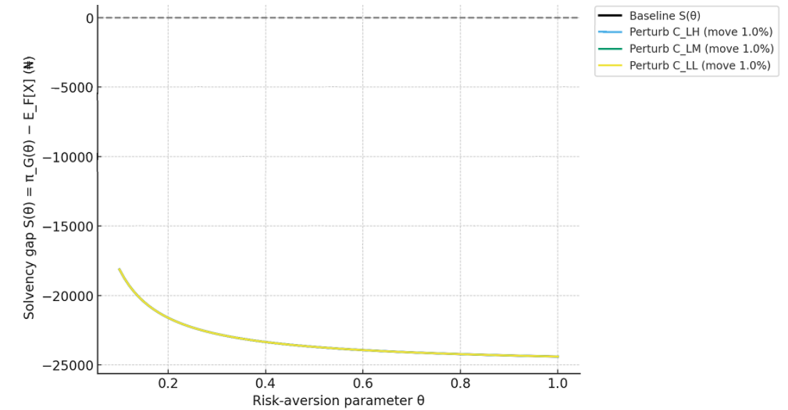
Figure 7: Solvency Sensitivity (Small Targeted C_{ij} Perturbations)
