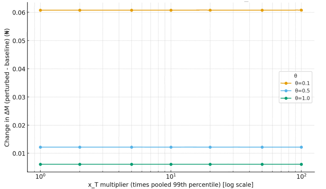
Figure 8: Tail Risk Sensitivity – relocating \varepsilon - mass to Extreme Loss x_T
