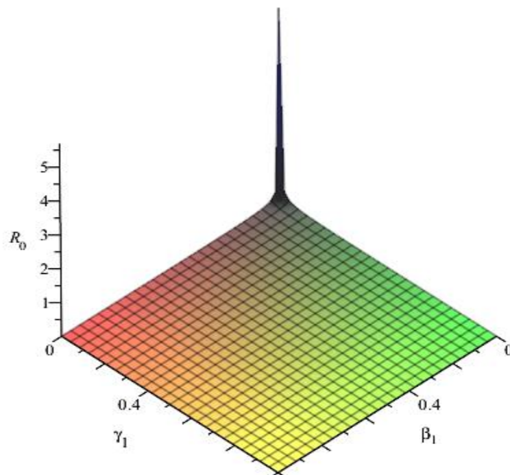
Fig. 3: Sensitivity of the basic reproduction number to the parameters \gamma_1 and \beta_1
