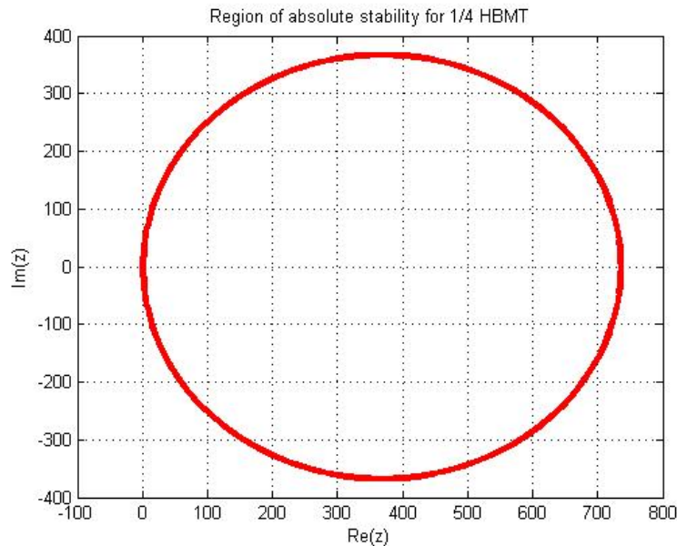
Figure 1: Region of absolute stability of \frac{1}{4} HBM
