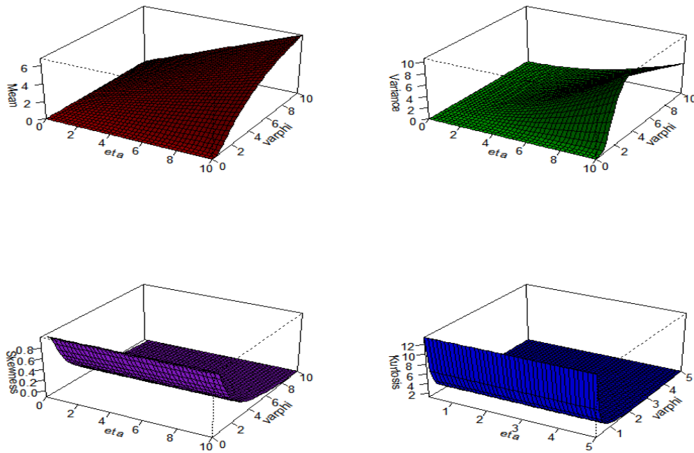
Figure 3: 3D plots of mean, variance, skewness and kurtosis for the APGOGEW
