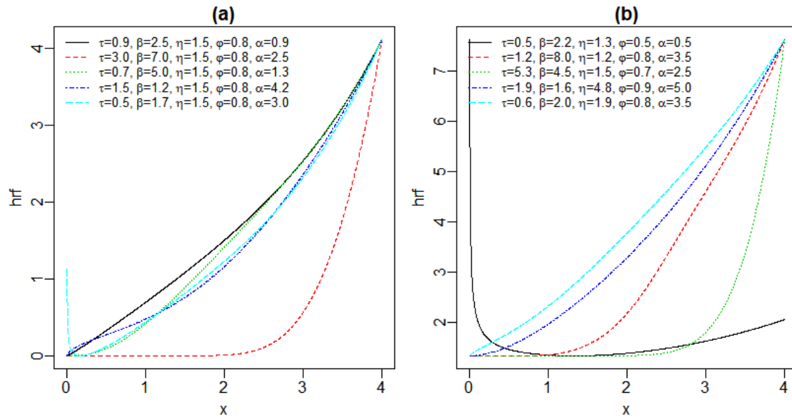
Figure 2: HRF plots of X \sim \text{APGOGEW}(\alpha, \beta, \tau, \eta, \varphi) .
