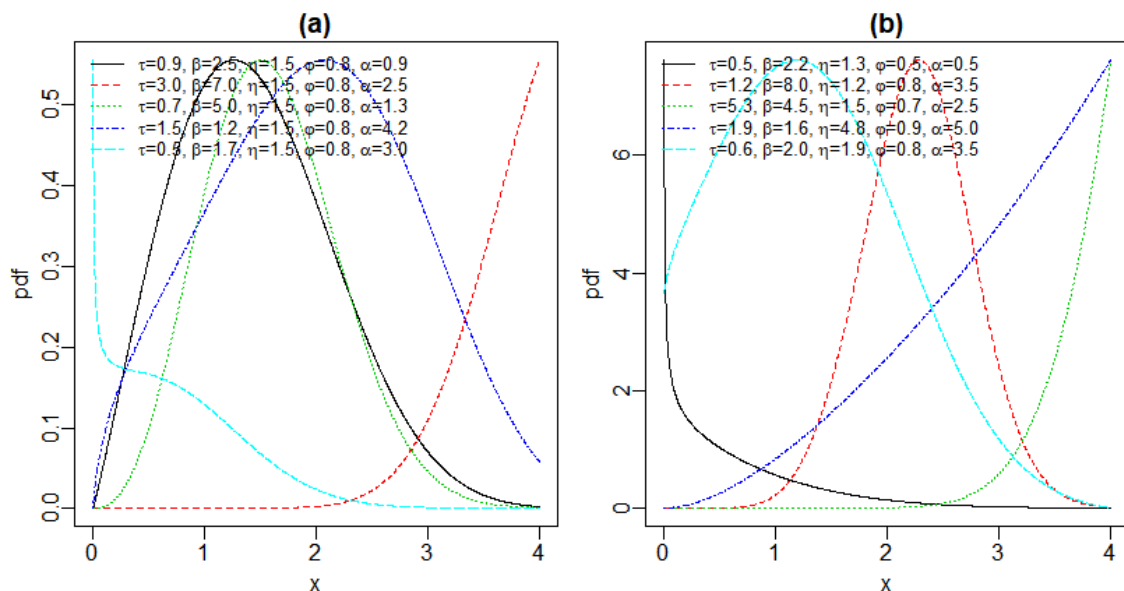
Figure 1: PDF plots of X \sim APGOGew(\alpha, \beta, \tau, \eta, \varphi) .
