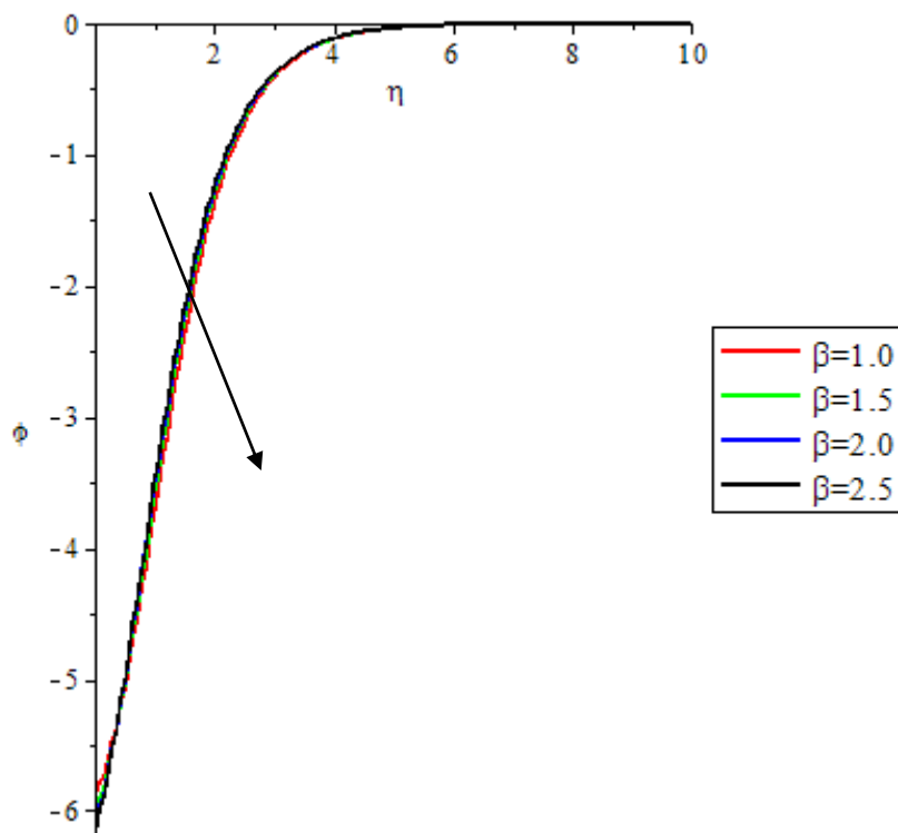
Figure 4.8: Graph of \varphi(\eta) for various values of \beta .
