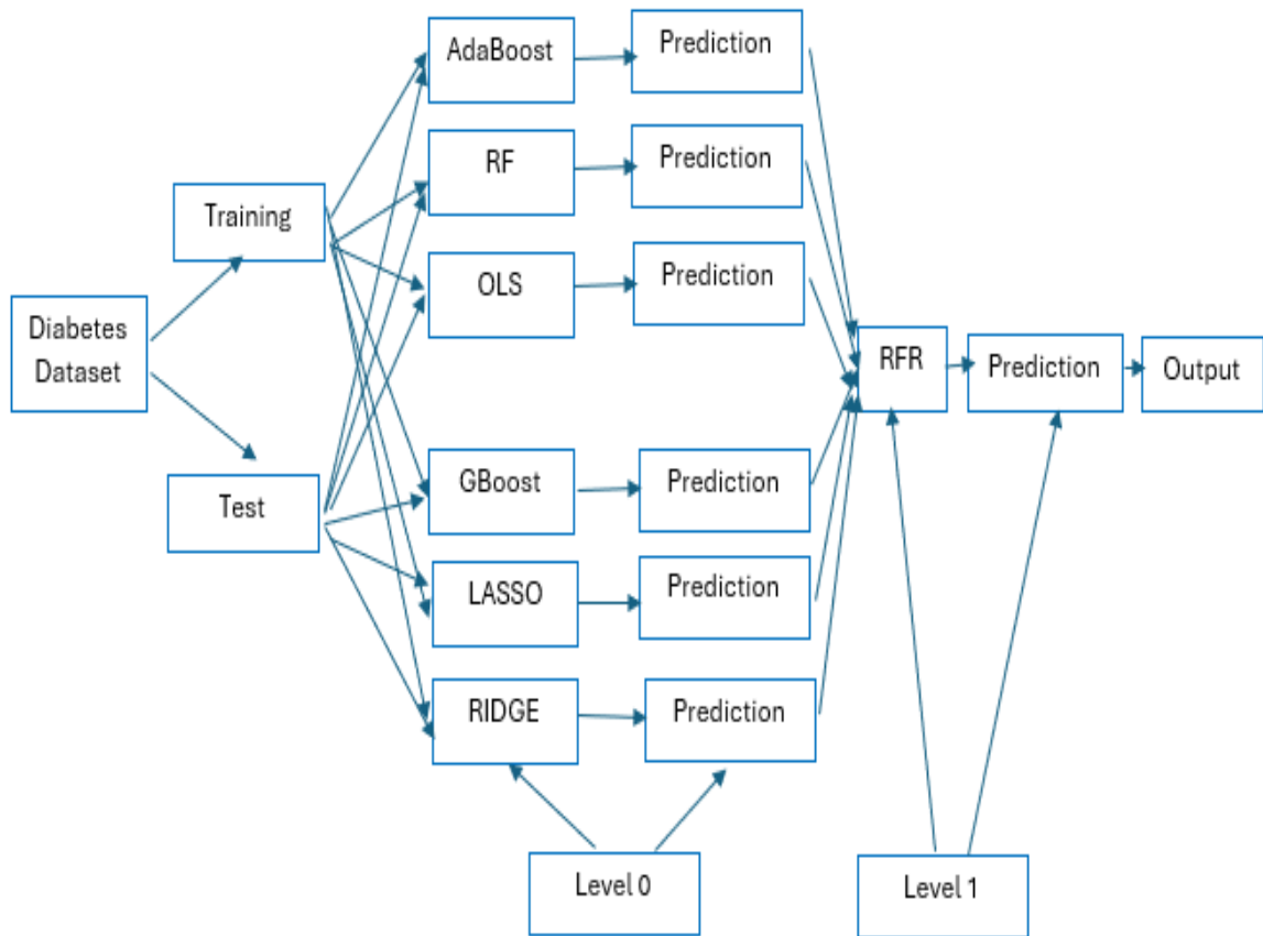
Figure 1: Proposed Architecture for Stacking Ensemble Learning
