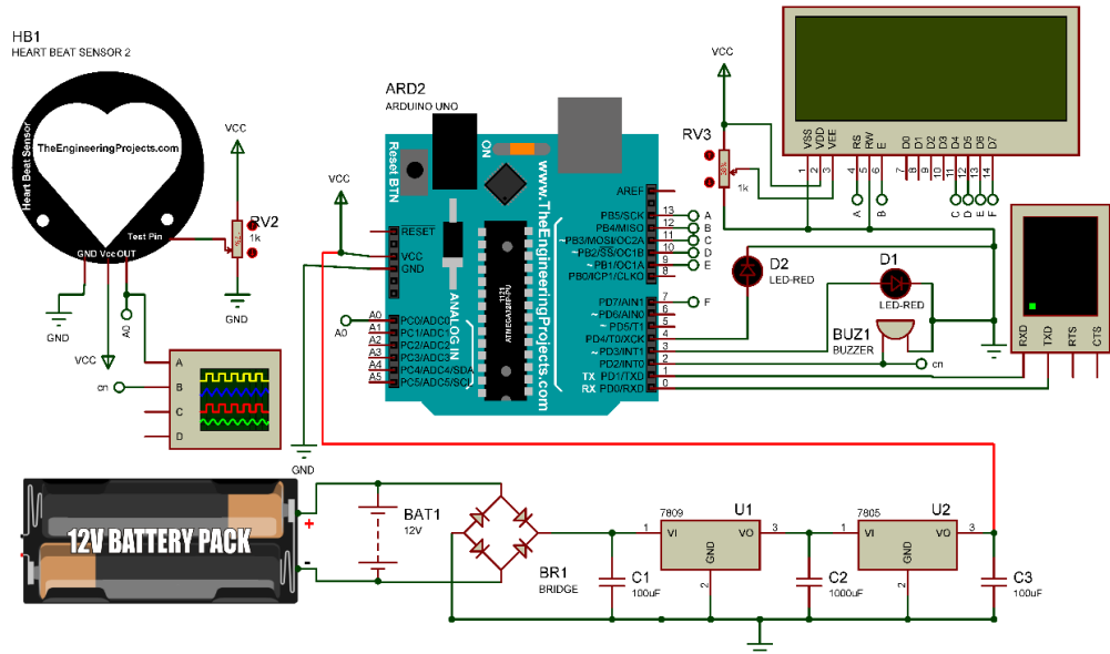
Figure 5: Simulated Circuit Diagram of the Heartbeat Monitoring System in Proteus
