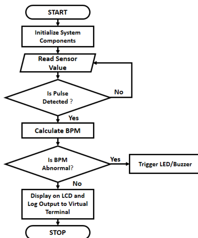
Figure 7: Flowchart of the Heartbeat Monitoring System
