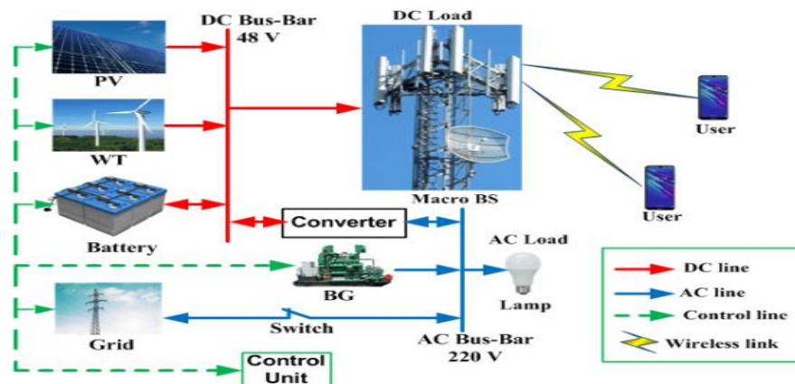
Figure 3: System Architecture
