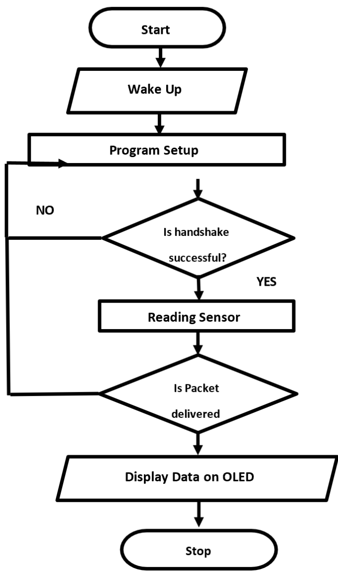
Figure 10. Flowchart of Wireless Access Point client
