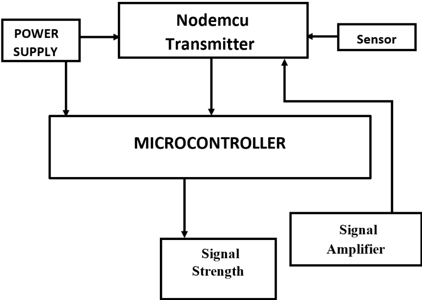
Figure 2. System block diagram of transmitter
