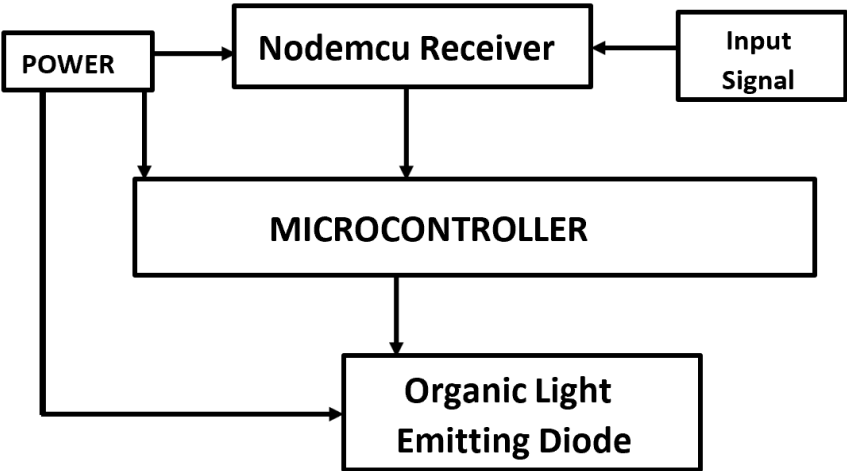
Figure 3. System block diagram of receiver
