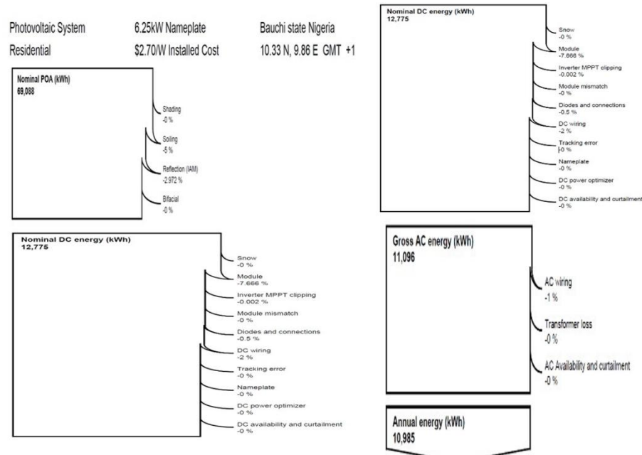
Figure 11: General losses in conversion process
