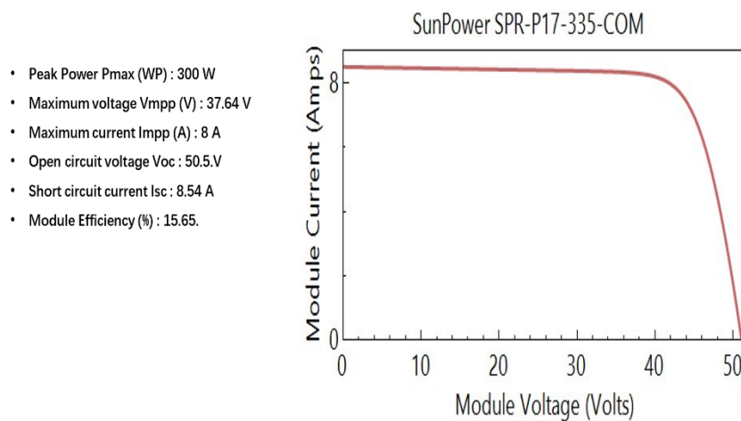
Figure 3: I_V curve(current/voltage)
