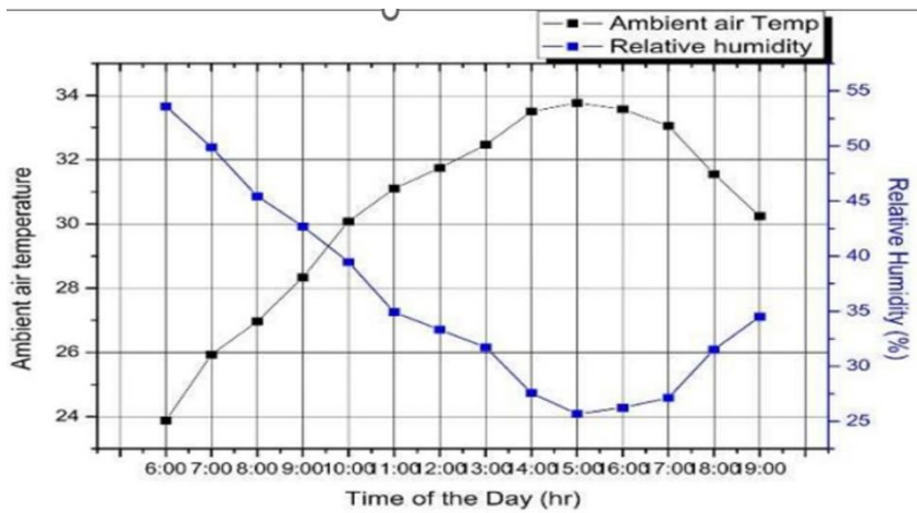
Figure 13: Hourly variation of the ambient air temperture
