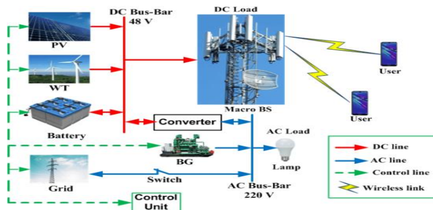
Figure 3: System Architecture
