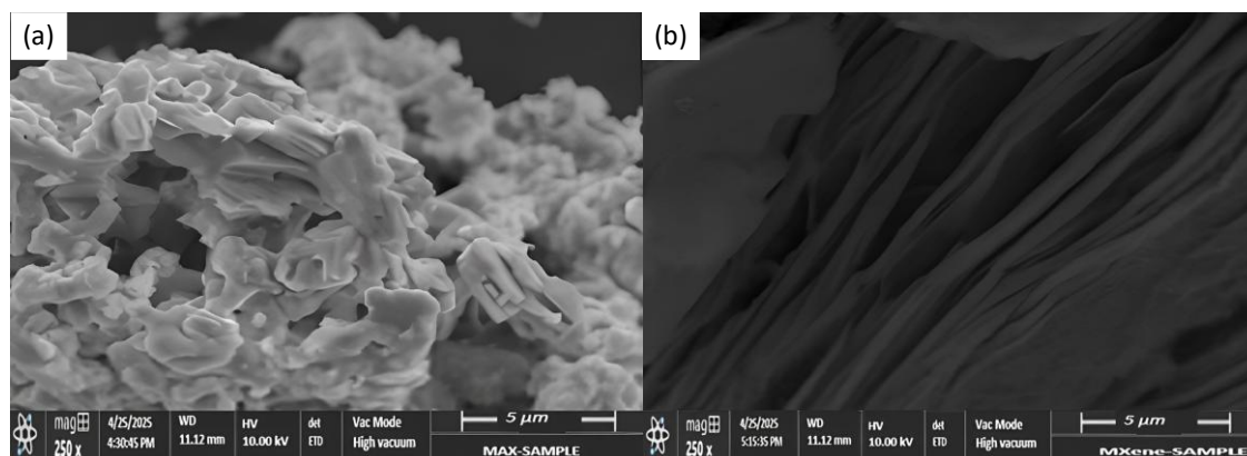
Figure 2. SEM Images (a) \text{Ti}_3\text{AlC}_2 MAX Phase (b) \text{Ti}_3\text{C}_2\text{T}_x MXene
