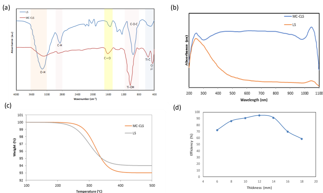
Figure 8. (a) FTIR Spectra of LS & MC-CLS; (b) UV-Visible Spectra of LS & MC-CLS; (c) TGA curves of LS and MC-CLS and (d) Evaporation efficiency at different thickness
