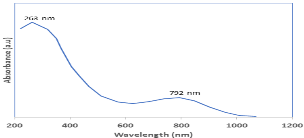
Figure 6. UV-VIS Absorption spectra of \text{Ti}_3\text{C}_2\text{T}_x MXene
