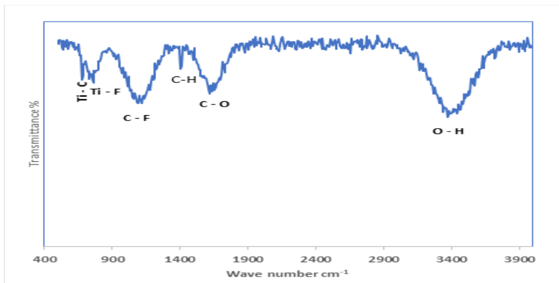
Figure 5. FTIR of \text{Ti}_3\text{C}_2\text{T}_x MXene
