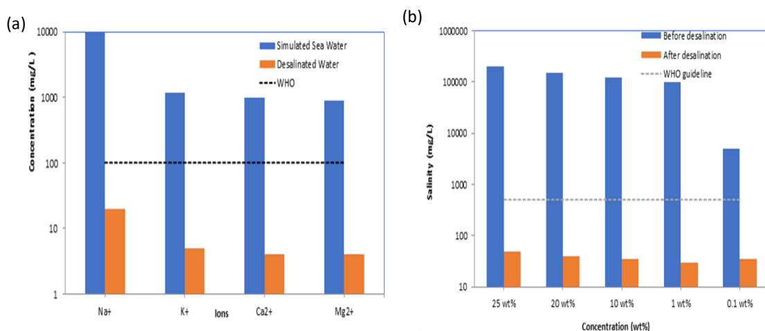
Figure 11. (a) Concentration of ions and (b) Salinity in different brine samples before and after desalination. The dashed line demoted the World Health Organization (WHO) standard of ions and salinity for drinking water.
