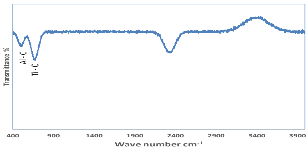
Figure 4. FTIR of \text{Ti}_3\text{AlC}_2 MAX Phase
