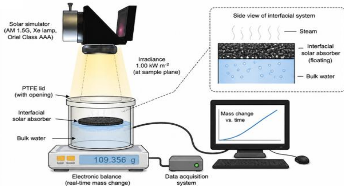
Figure 1. Schematic diagram of the laboratory setup for solar evaporation evaluation
