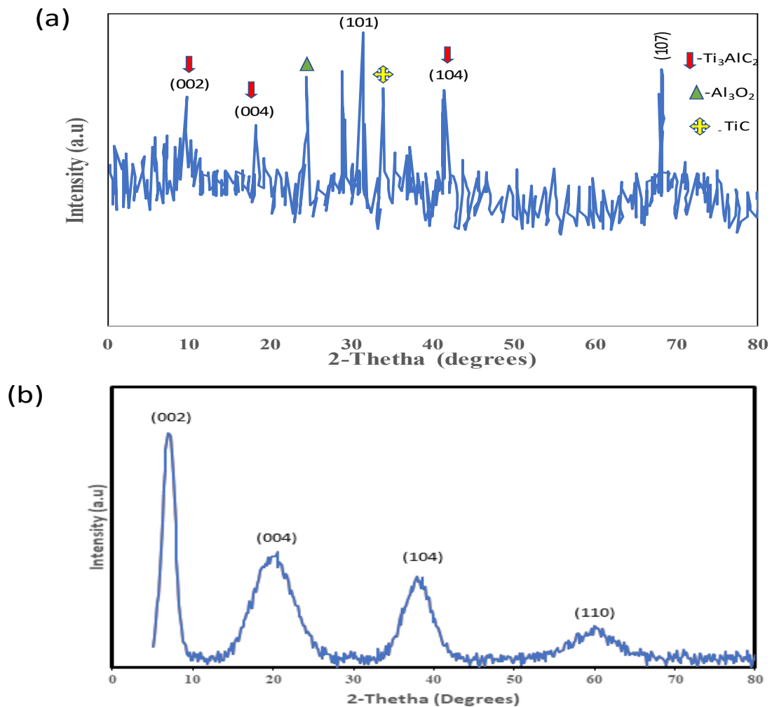
Figure 3. XRD of (a) \text{Ti}_3\text{AlC}_2 MAX Phase; (b) \text{Ti}_3\text{C}_2\text{T}_x MXene
