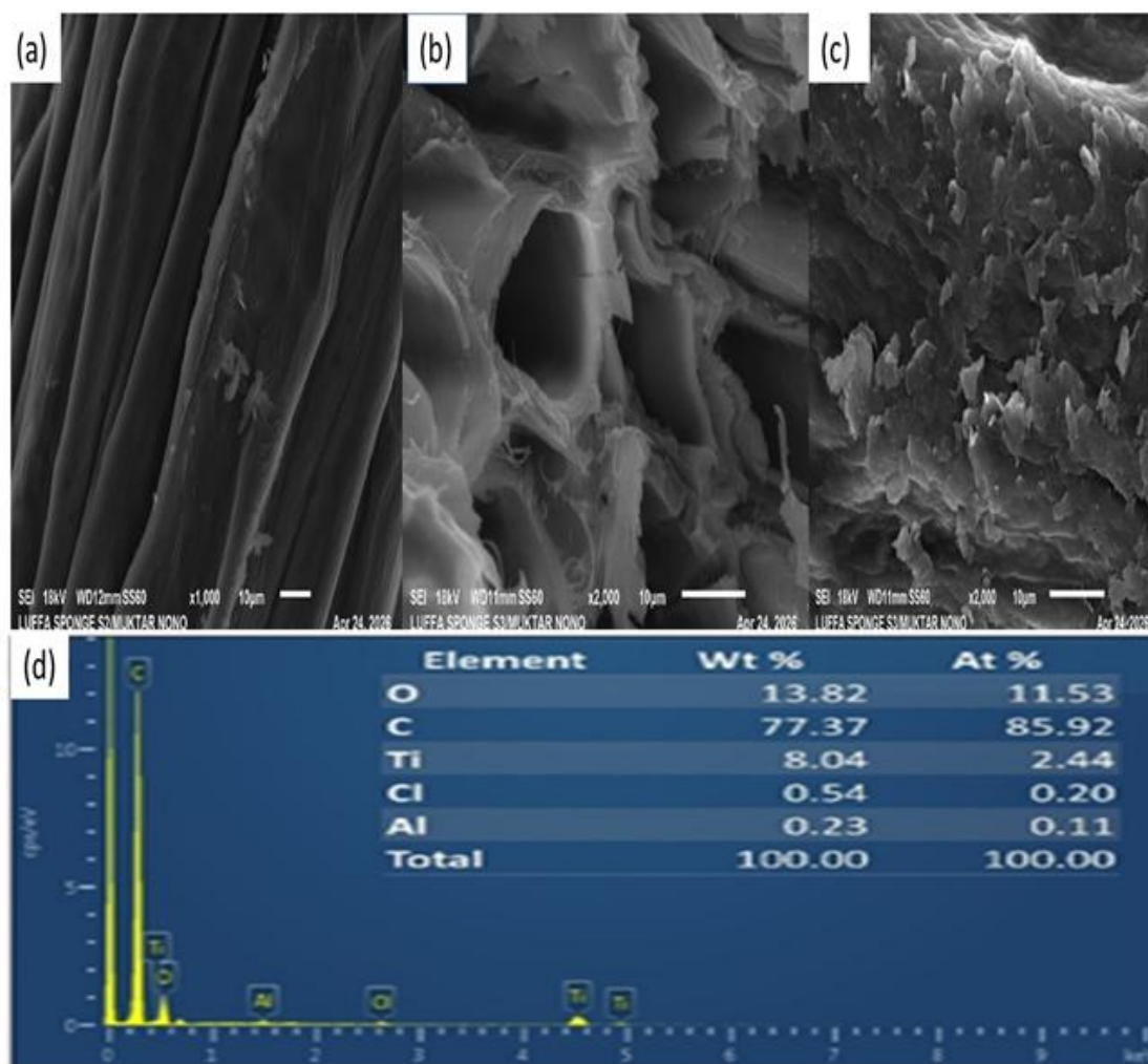
Figure 7. SEM micrographs of (a) pristine luffa sponge (LS), (b) cross-section of LS, (c) MXene-coated carbonized luffa sponge (MC-CLS), and (d) EDX spectrum and elemental mapping of MC-CLS.
